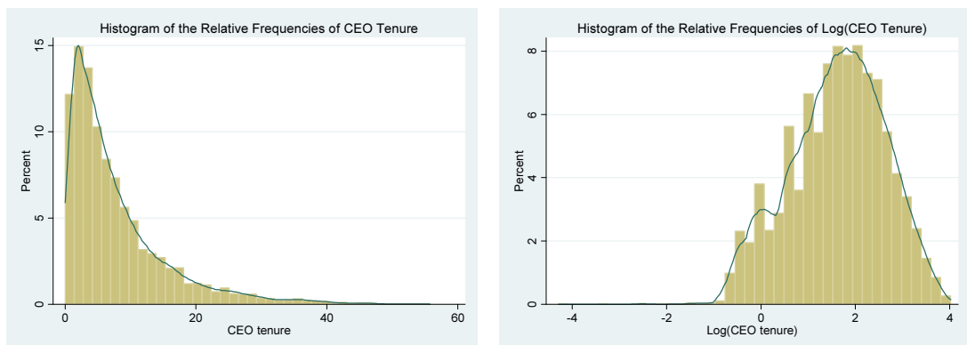
Figure 1. Histograms of the Relative Frequencies of CEO Tenure and the Log of CEO Tenure
